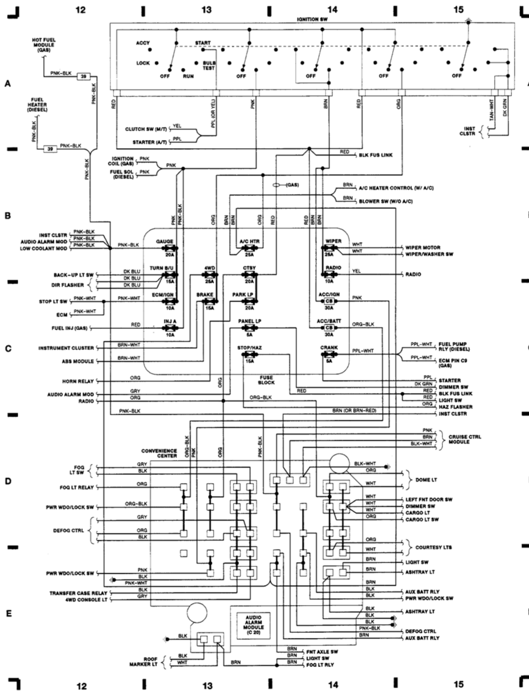
Fig. 4: Fuse Block
