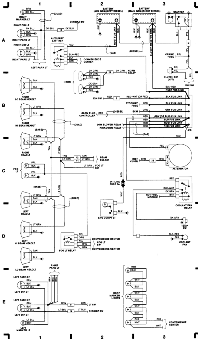
Fig. 1: Engine Compartment & Headlights
